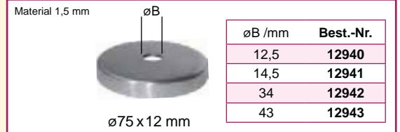
Abdeckrosetten / Rosaces Cover plates / Copriflange / Rozetler
