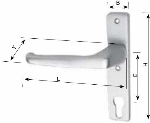
Best.-Nr. B-290/20-HD L x T = 135 x 55 mm B x H = 32 x 204 mm E = 92 mm,
